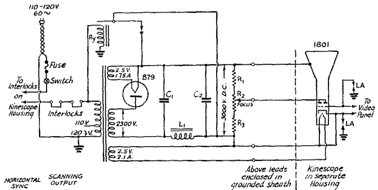
Fig. 5 — Power supply circuit for the 1801.
