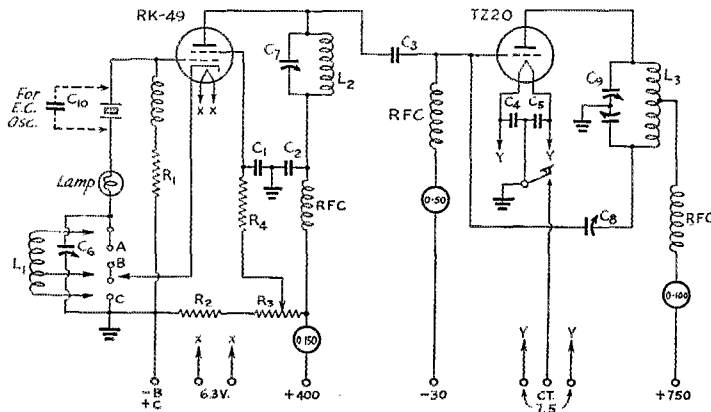
Fig. 1 — Circuit diagram of the two-tube six-band transmitter.
